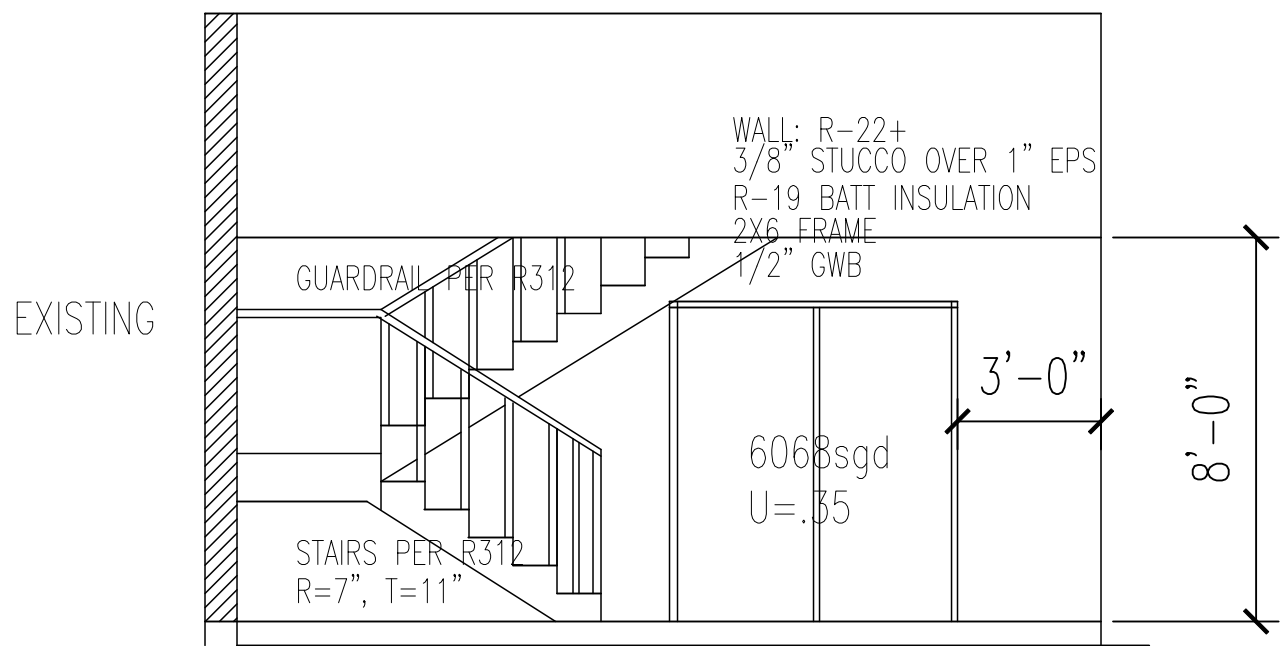
east elevation
