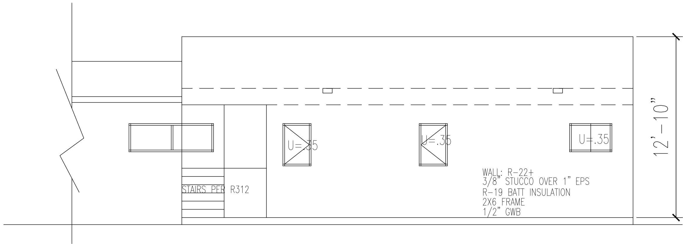
north elevation
