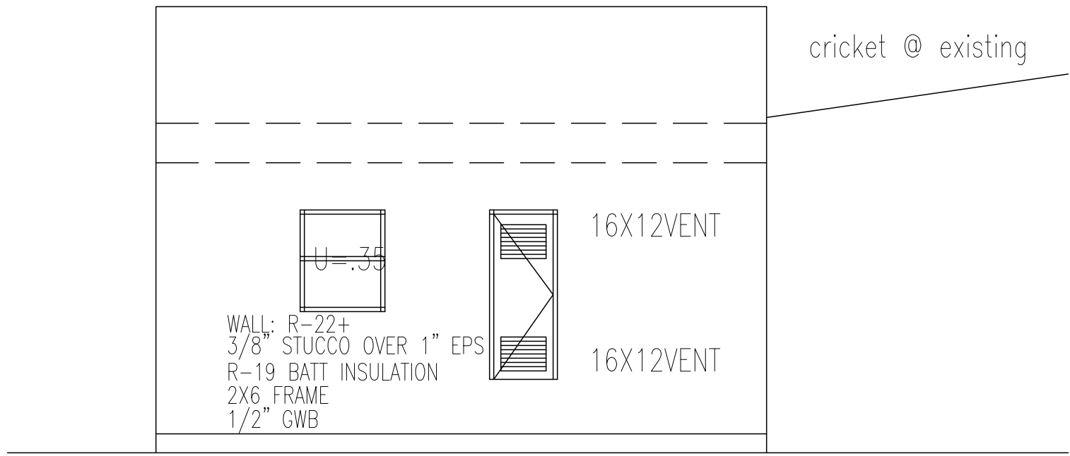
WEST elevation
